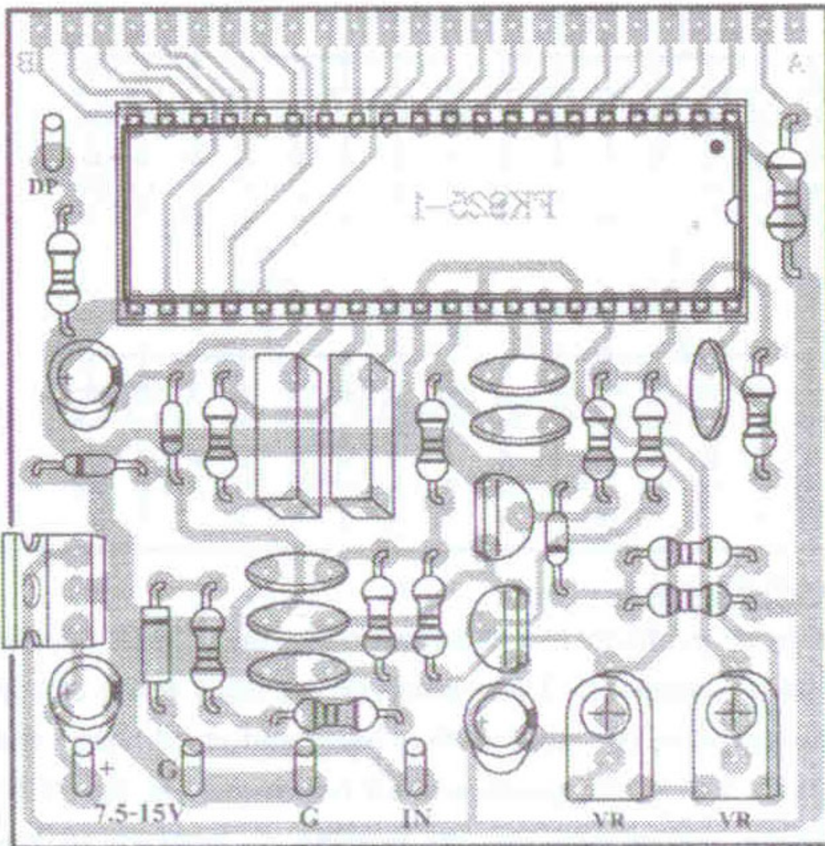
Figure 3. Connections FK925-1
