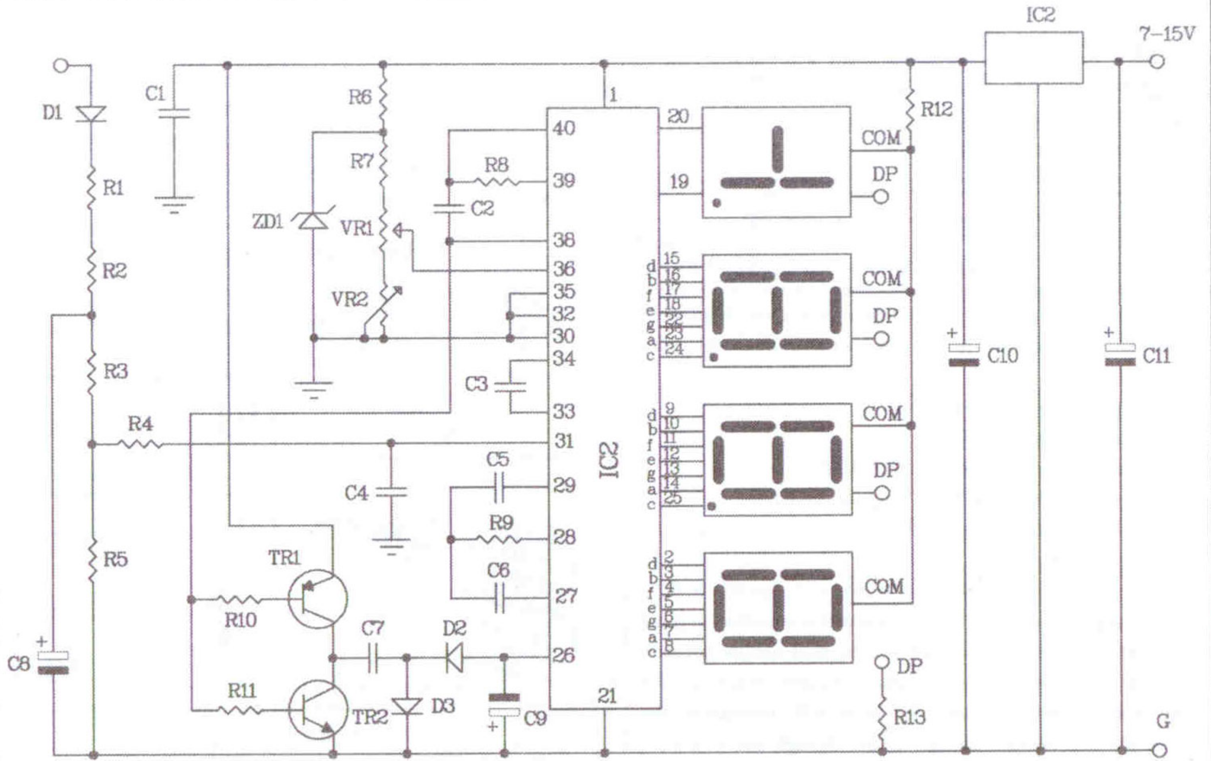
Figure 2. The digital AC voltmeter circuit
