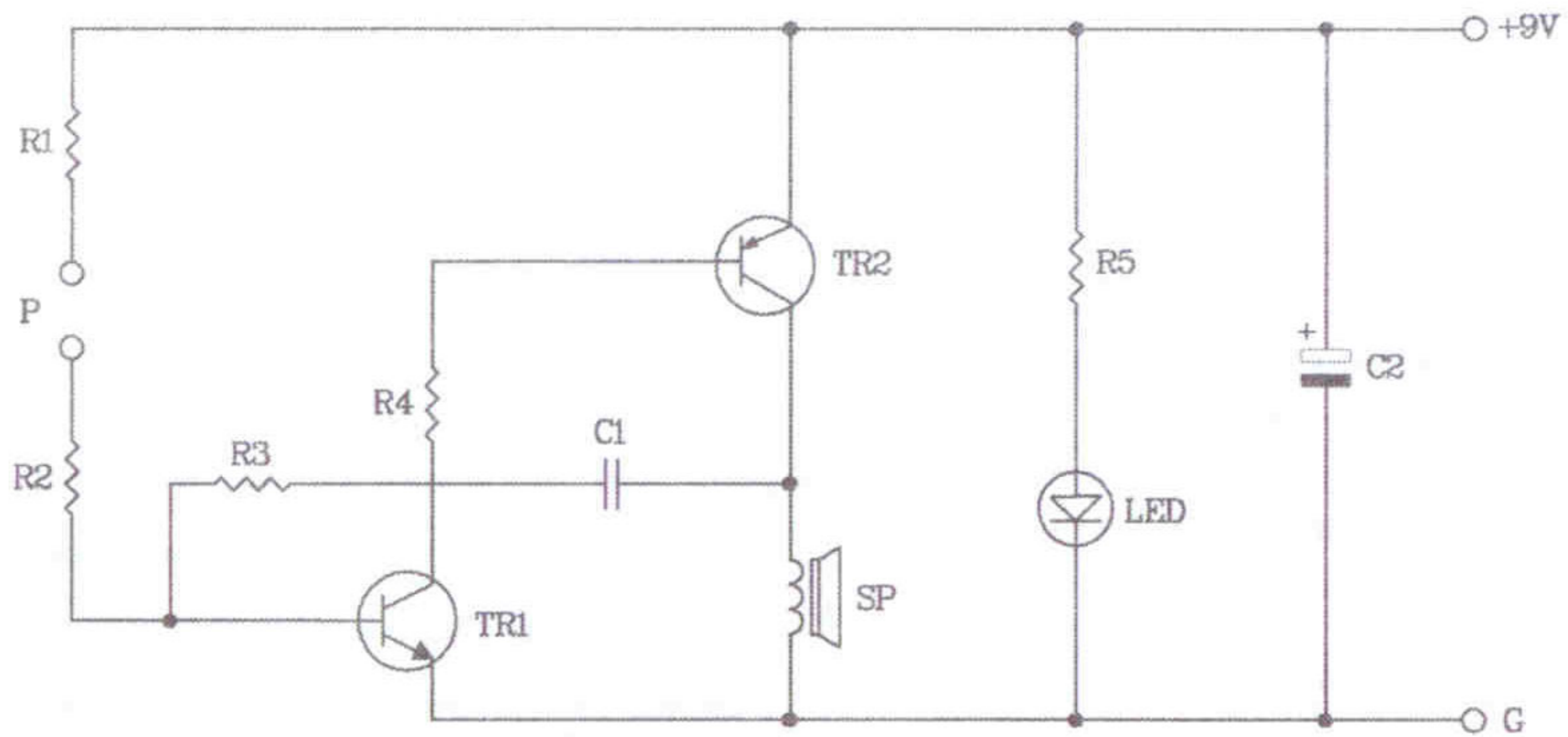
Figure 2. The continuity meter circuit
