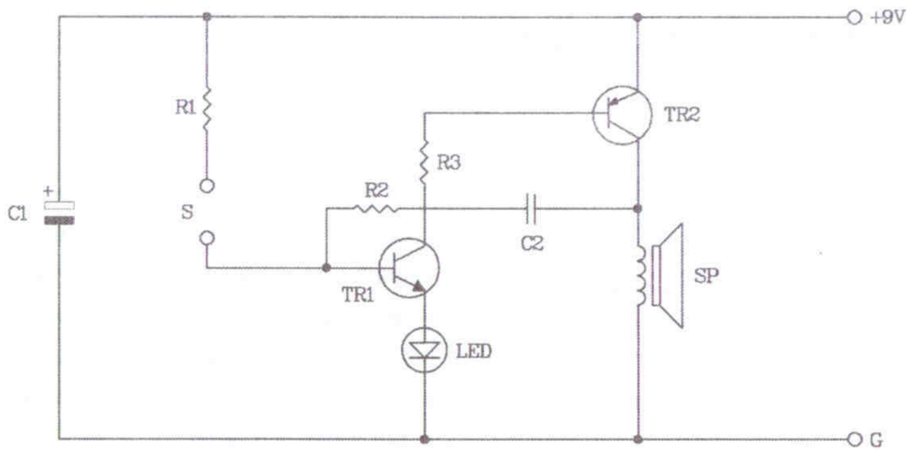
Figure 2. The raining alarm circuit
