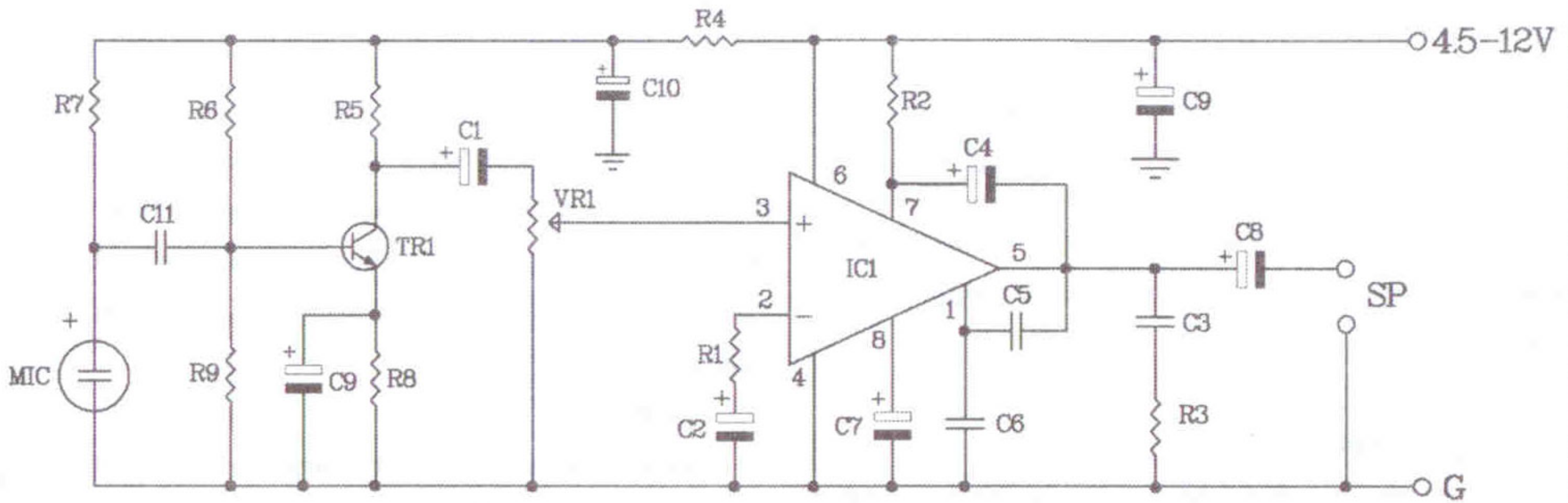
Figure 2. The mini megaphone circuit
