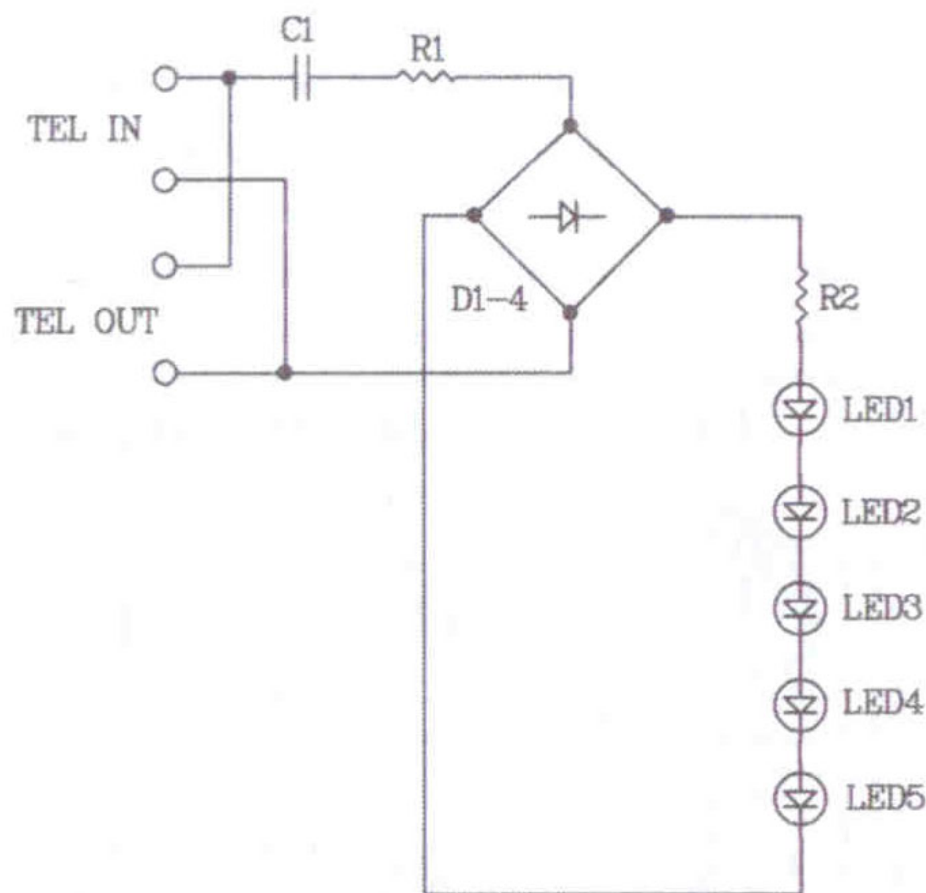
Figure 2. The ringing signal light 5 LED circuit
