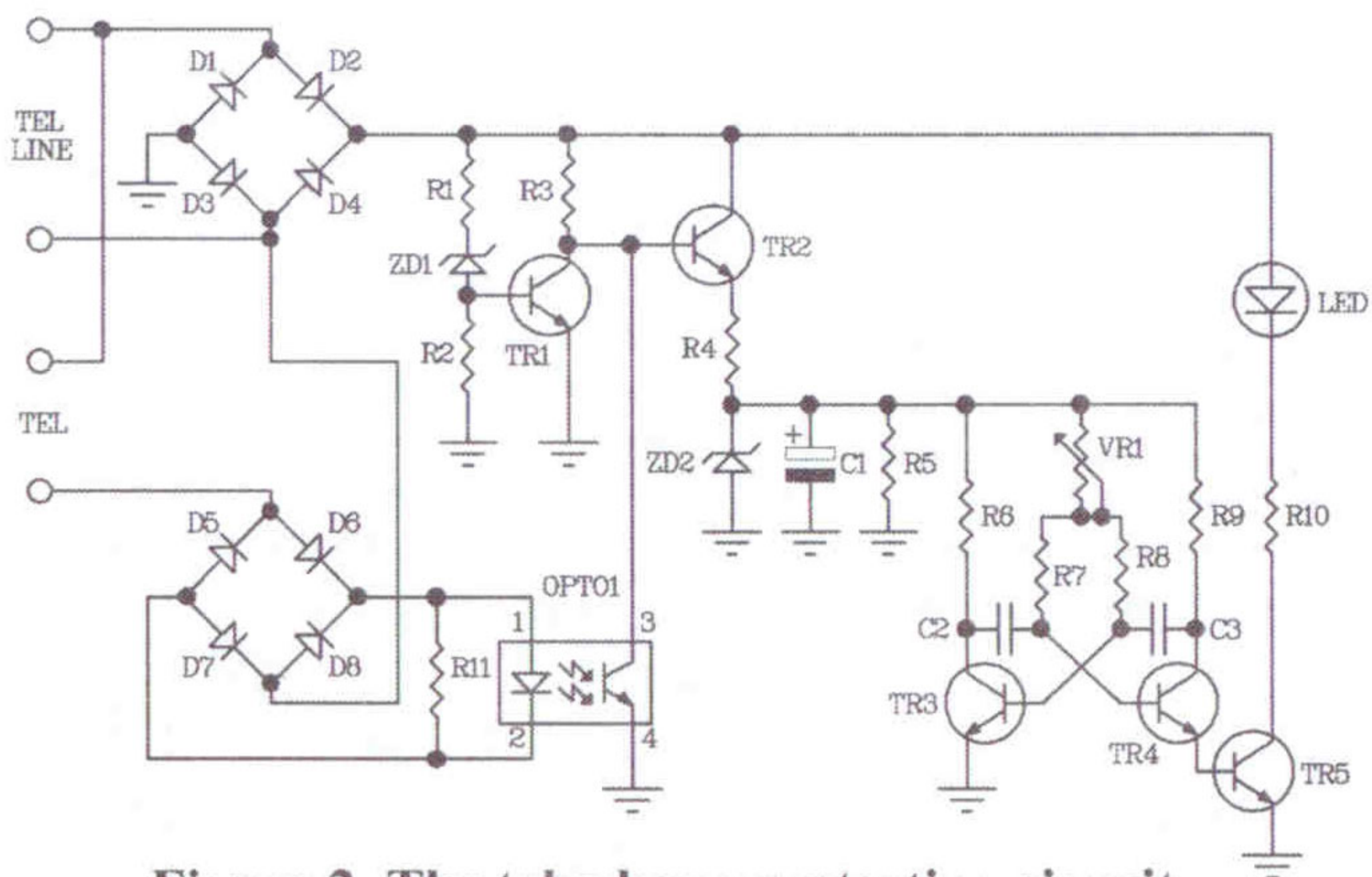
Figure 2. The telephone protection circuit
