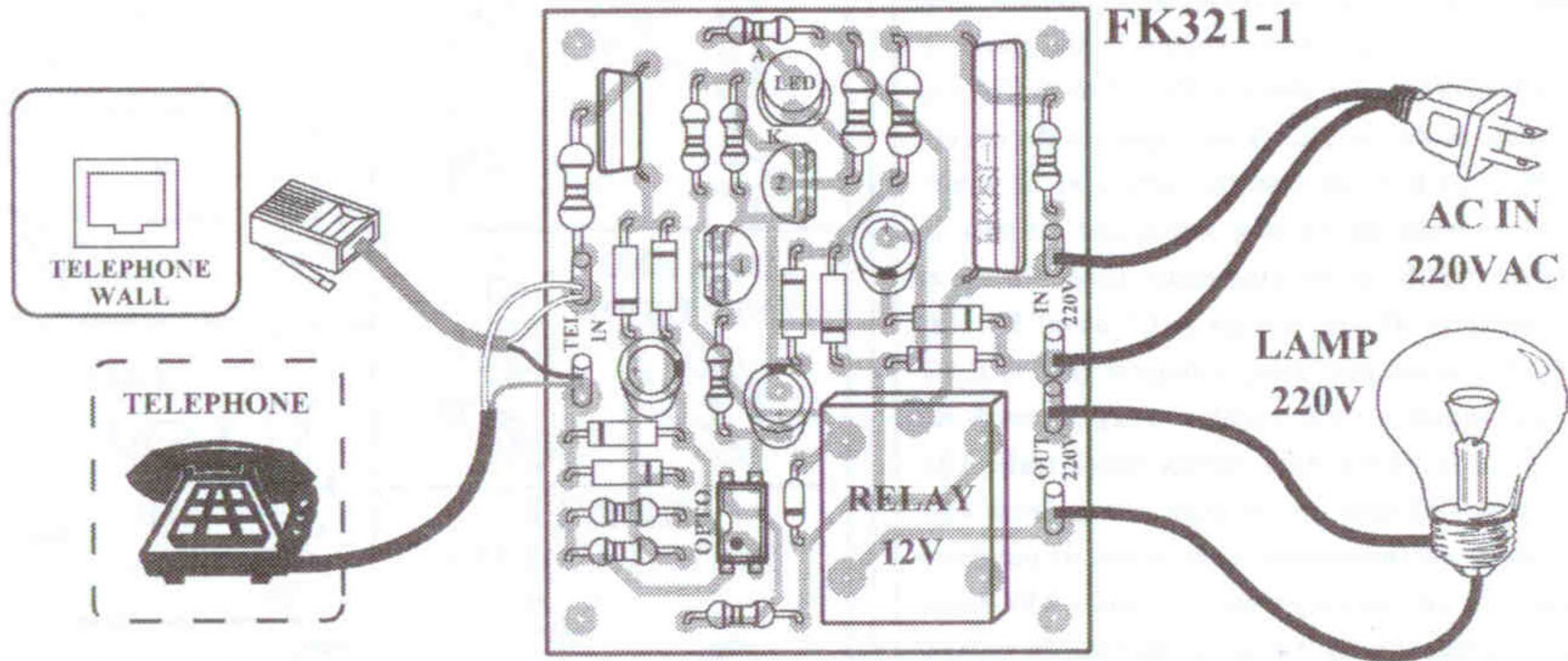
Figure 3. Connections
