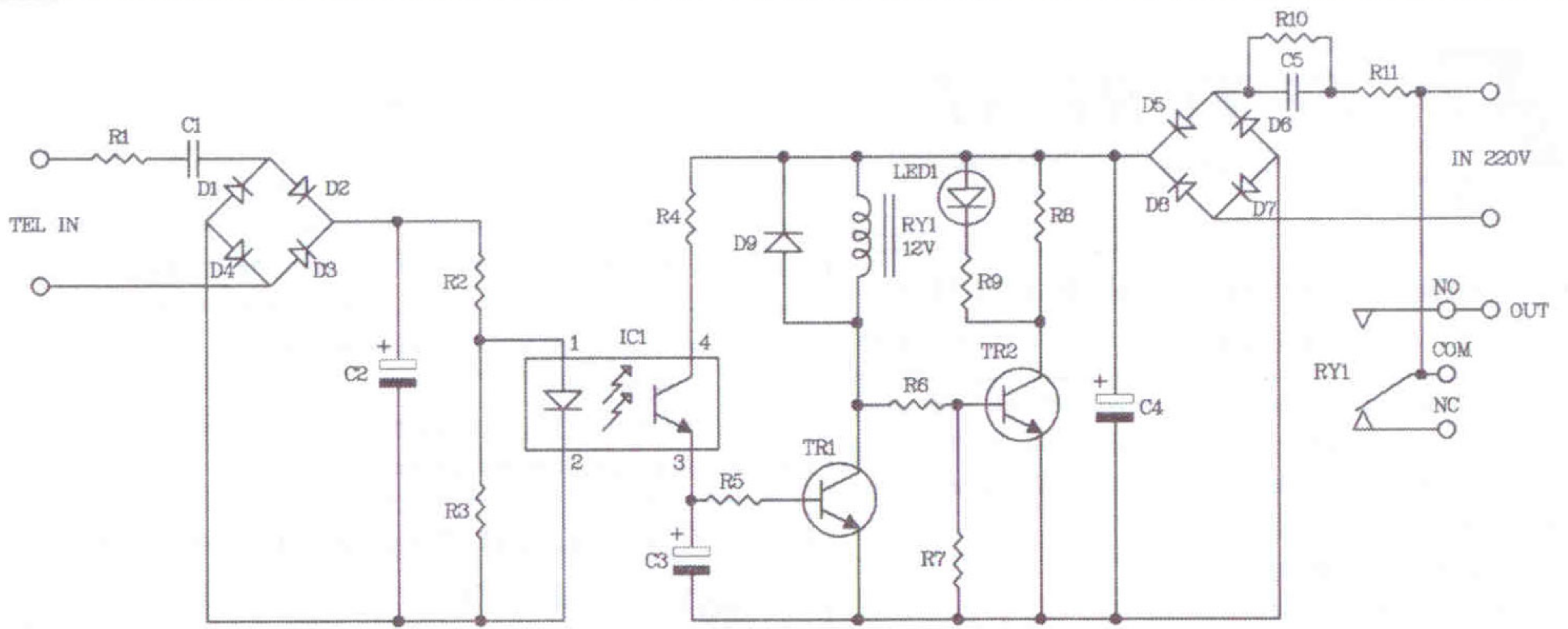
Figure 2. The phone ring signal light circuit
