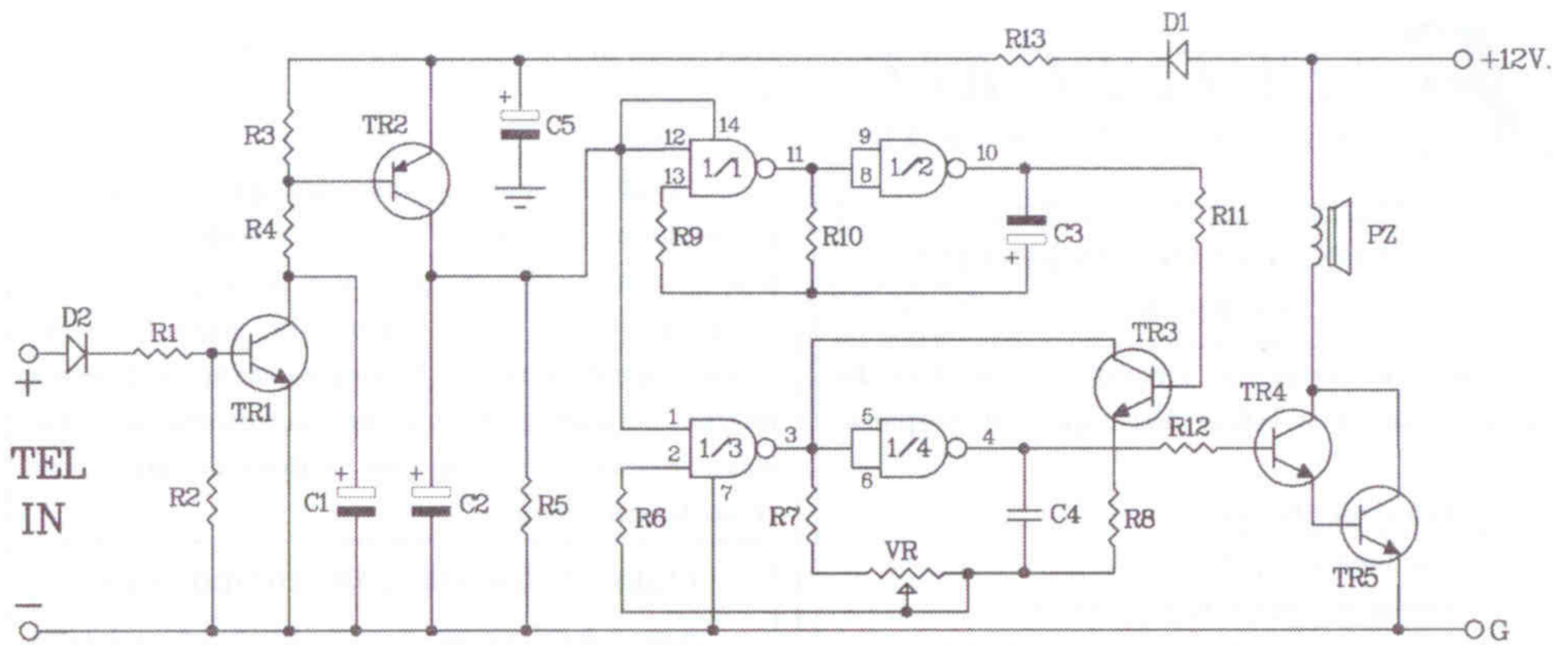
Figure 2. The high power telephone ringing 10W. circuit
