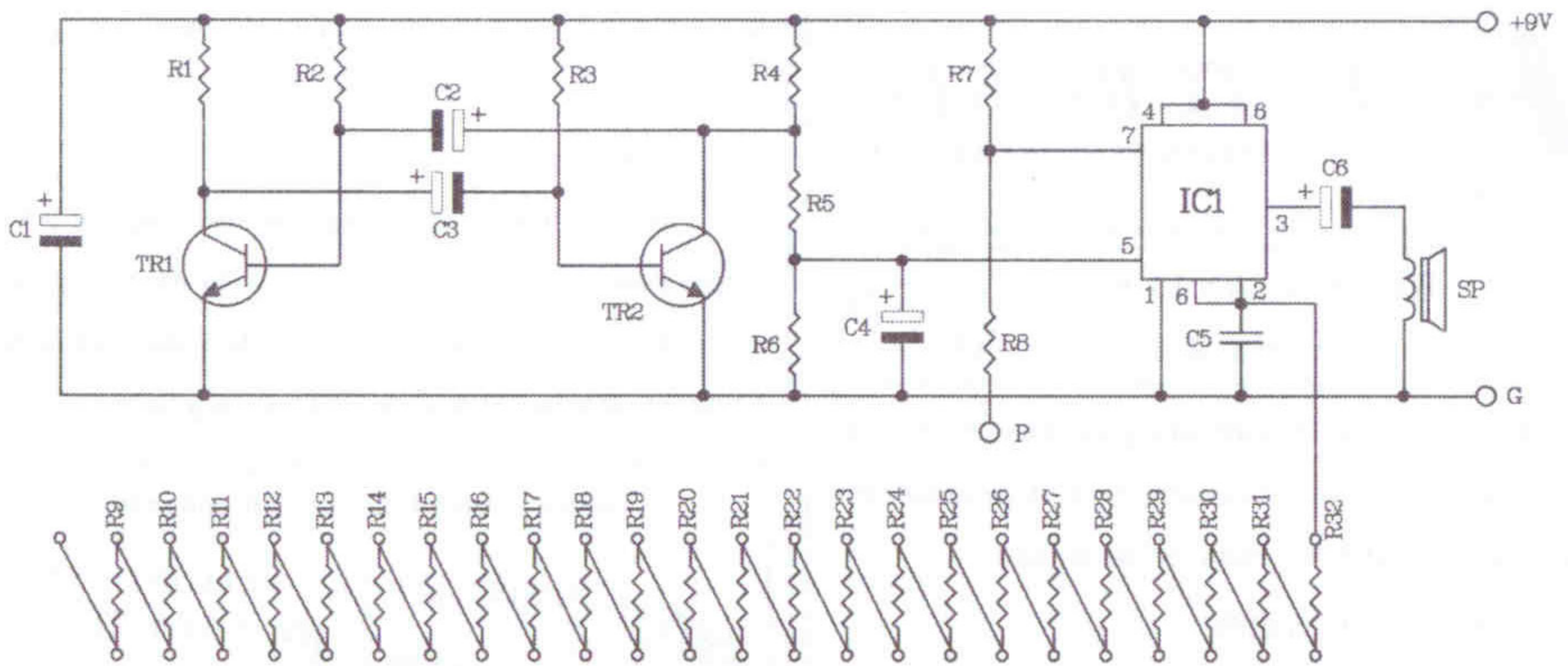
Figure 2. The melody organ 25 tone circuit
