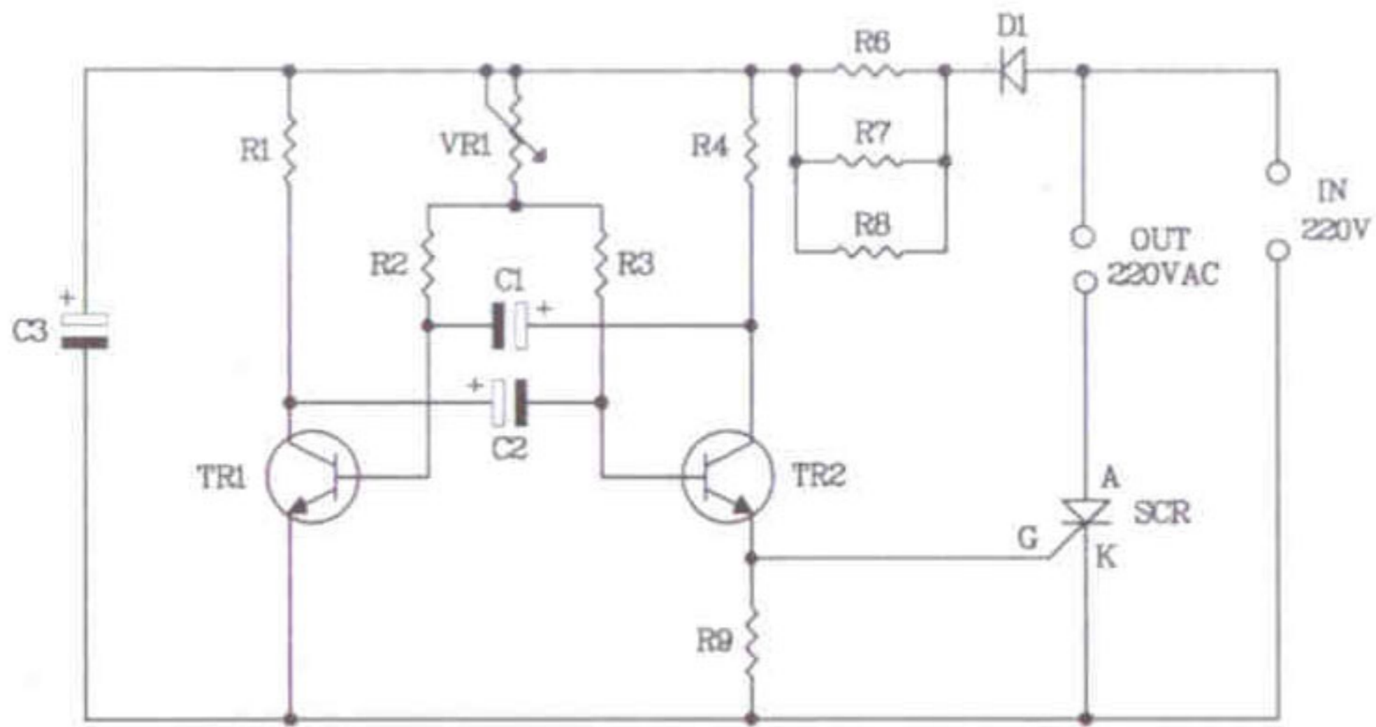
Figure 2. The AC flasher 1 CH. 700W. circuit
