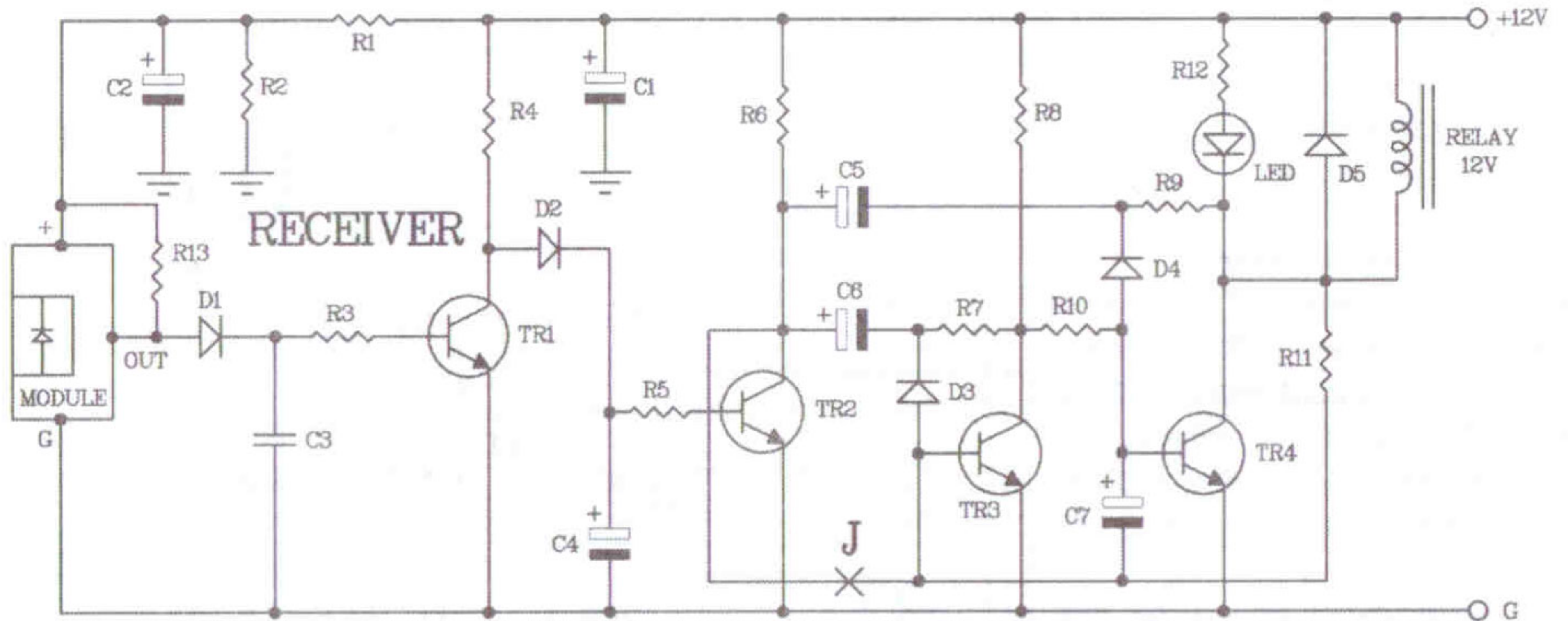
Figure 2. The infrared remote control 50' 1 ch. circuit
