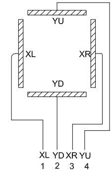
Circuit Diagram
